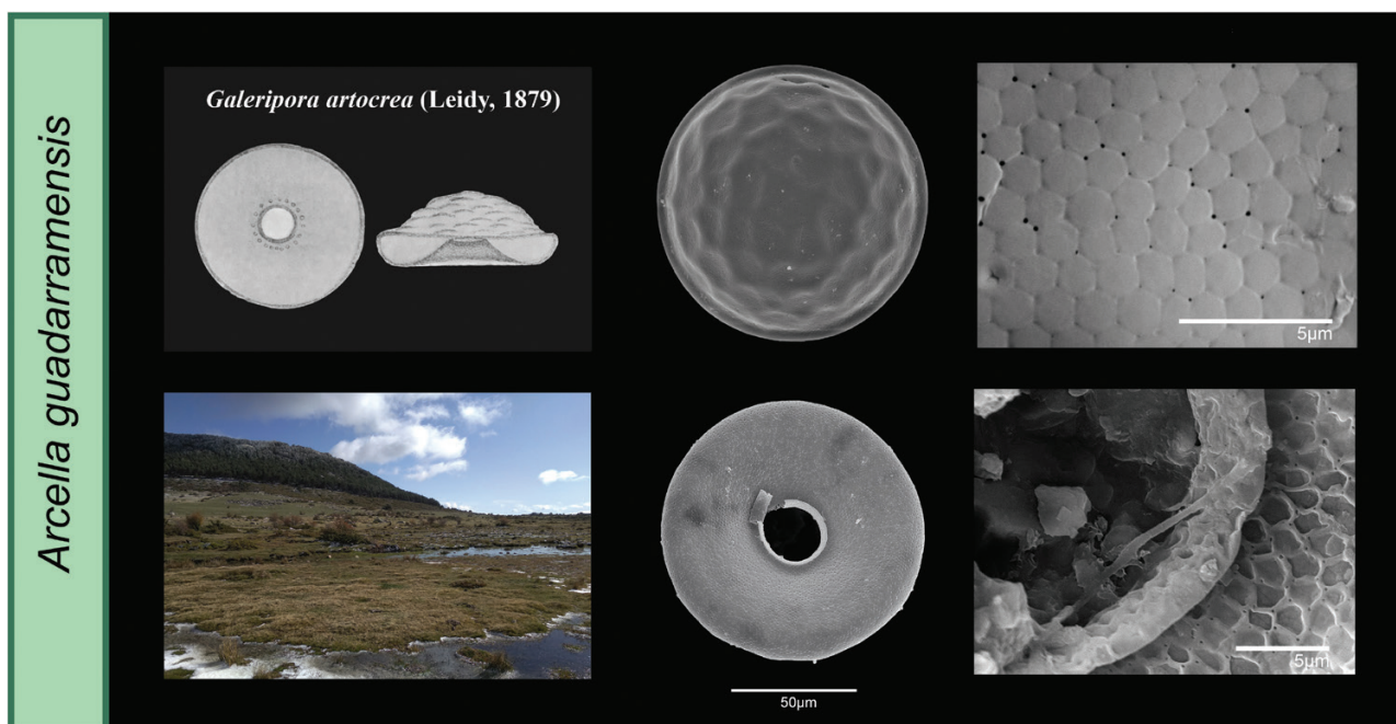
Figure 8. Arcella guadarrensis : scanning electron micrographs of the aboral and oral sides of the test. The images on the right represent a detail of the test and the structure of the aperture. On the left, a photograph of a typical habitat for this species, and original drawing of the closest resembling species, Galeripora artocrea (Leidy, 1879).
