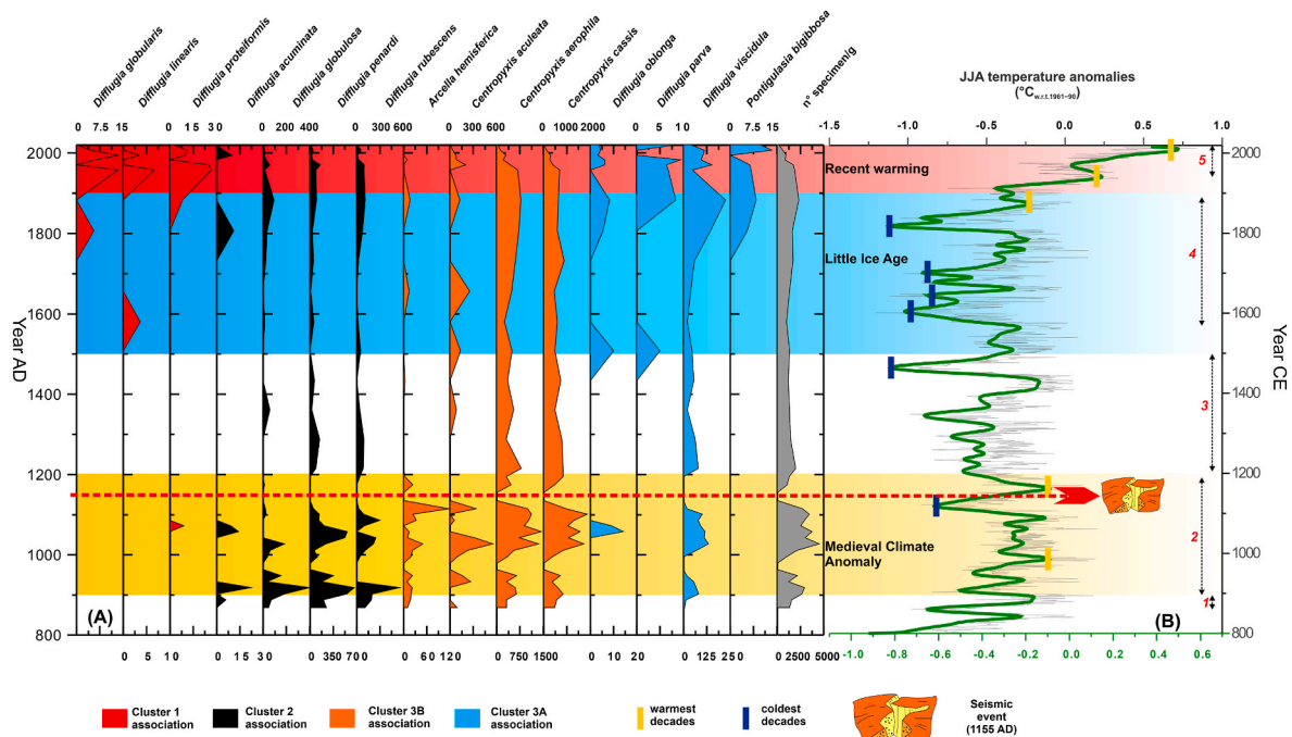
Fig. 9. Distribution of testate amoebae species ( \text{ind g}^{-1} ) along the sediment core of the Upper Balma Lake (A). Groups of the sediment core samples as highlighted by the Cluster associations are reported below the figure. Reconstructed temperatures from the European Alps (summer warmth between June and August JJA), with the orange and blue boxes denoting the 10 warmest and coldest decades respectively, and the smoothed green line being a 15-yr low-pass filter are reported in (B) (from Büntgen et al., 2006, 2016; Esper et al., 2024), modified. The red arrow indicates the possible seismic event recorded in 1155 AD near Lons-le-Saunier (Doubre et al., 2021). The numbers colored red on the right-hand side of the figure indicate the five intervals revealed by the testate amoebae. The colored bands (yellow, blue and red) mark the main climate phases in the last 1220 years. (For interpretation of the references to color in this figure legend, the reader is referred to the Web version of this article.)
