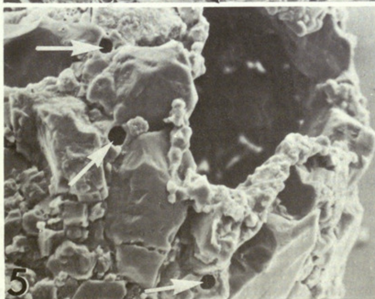
Figs 1–6 Diffflugia gramen Fig. 1 Lateral view \times 870 ; Fig. 2 View of aperture to show the irregular ridge (The arrows indicate the distance measured for the diameter of the aperture) \times 460 ; Fig. 3 Detail of aperture to indicate the ring of pores (arrowheads) \times 1000 ; Fig. 4 Detail of organic cement network \times 13000 ; Fig. 5 Side view of aperture to illustrate position of pores (white arrows) in relation to the apertural ridge \times 1450 ; Fig. 6 Part of shell surface to show distribution of organic cement \times 5300 .
